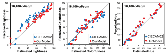
Figure 9: Comparison of the prediction of all 40 samples (estimated lightness using our model) for one particular phase (16,400 cd/m 2 ) against perceived lightness from the user study. It can be seen that our model achieves very good lightness, colorfulness and hue prediction. CIECAM02 is not able to predict lightness with the same accuracy.
