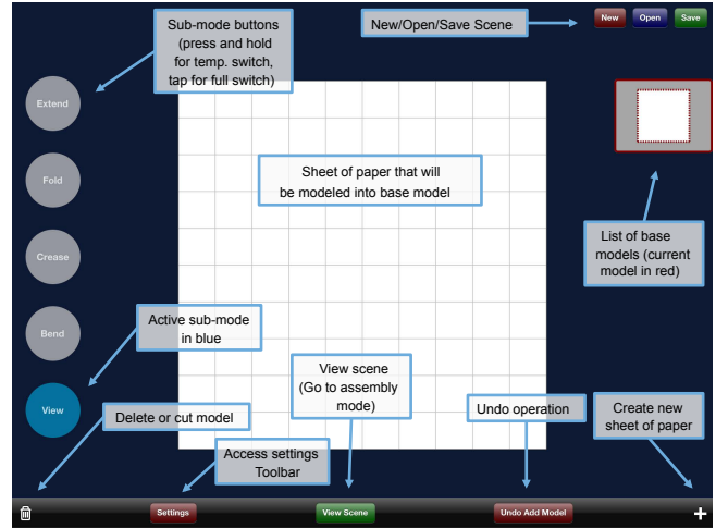
Figure 3. Interface for the modeling mode of Paper3D. Radio buttons (left) allow switching between submodes; the view sub-mode is active. Model thumbnails (right) are used to select/edit a different model. The bottom toolbar offers additional functionality such as undoing. The assembly mode interface has different submodes but an otherwise similar interface.
